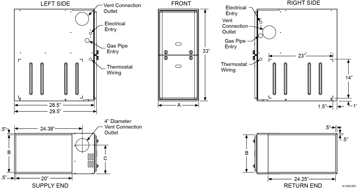
Figure 1: Dimensions
